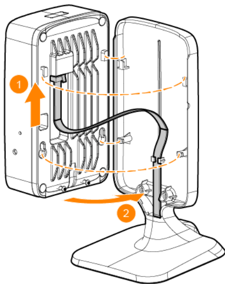
Figure 1 Installing Access Point to Mount Stand
