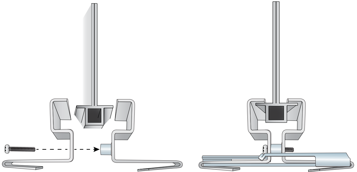
Figure 2 Attaching the AP-MNT-CM1 to a ceiling rail
