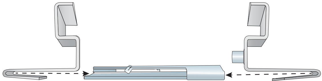
Figure 1 Attaching the ceiling rail brackets to the mounting plate
