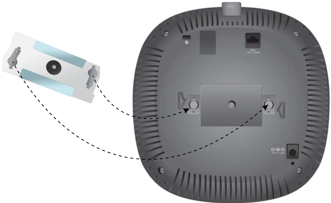
Figure 3 Securing the AP to the AP-MNT-CM1
